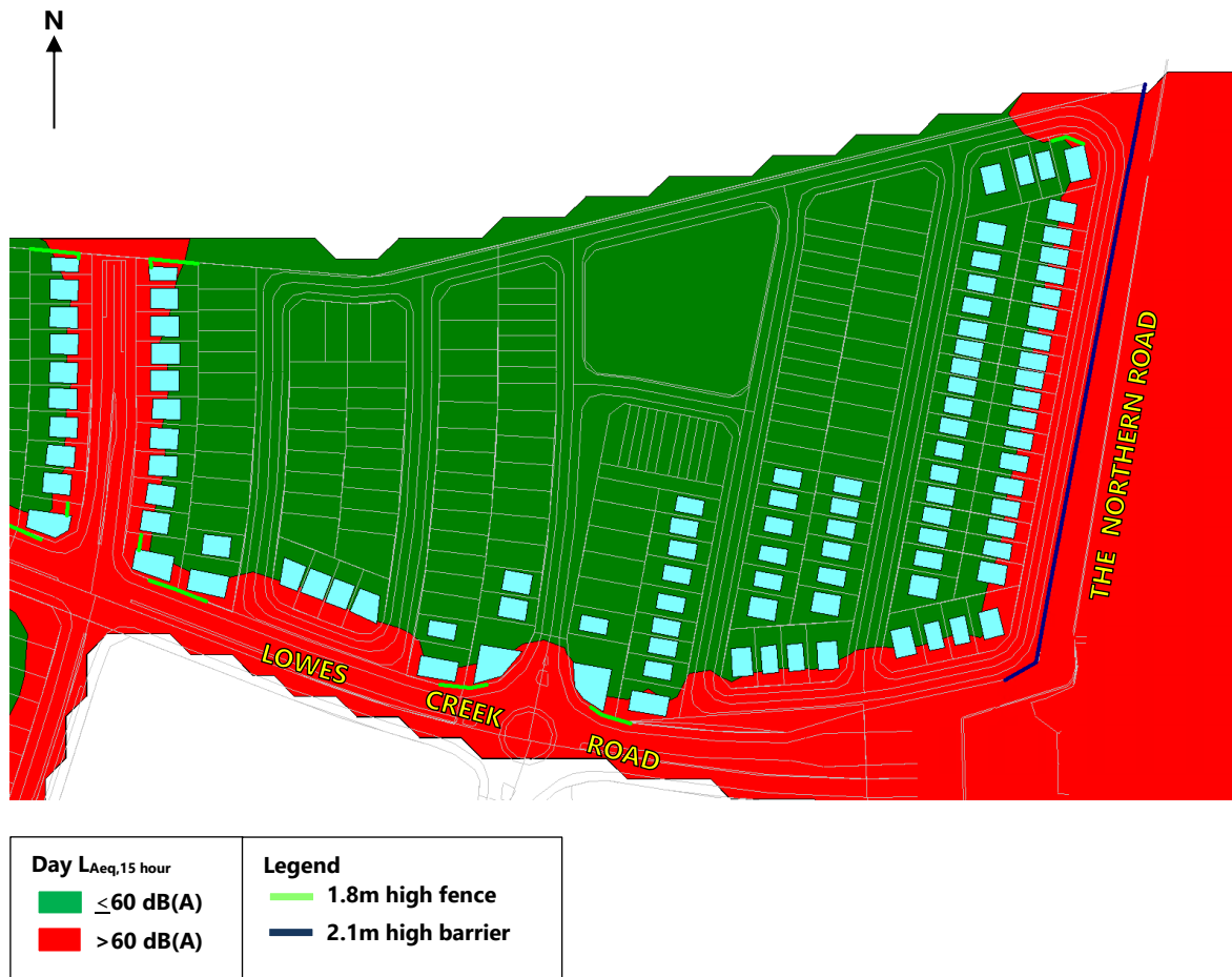
Figure 4 – Design Year 2031 Day Time L_{Aeq,15 \text{ hour}} Noise Contours (First Floor)
